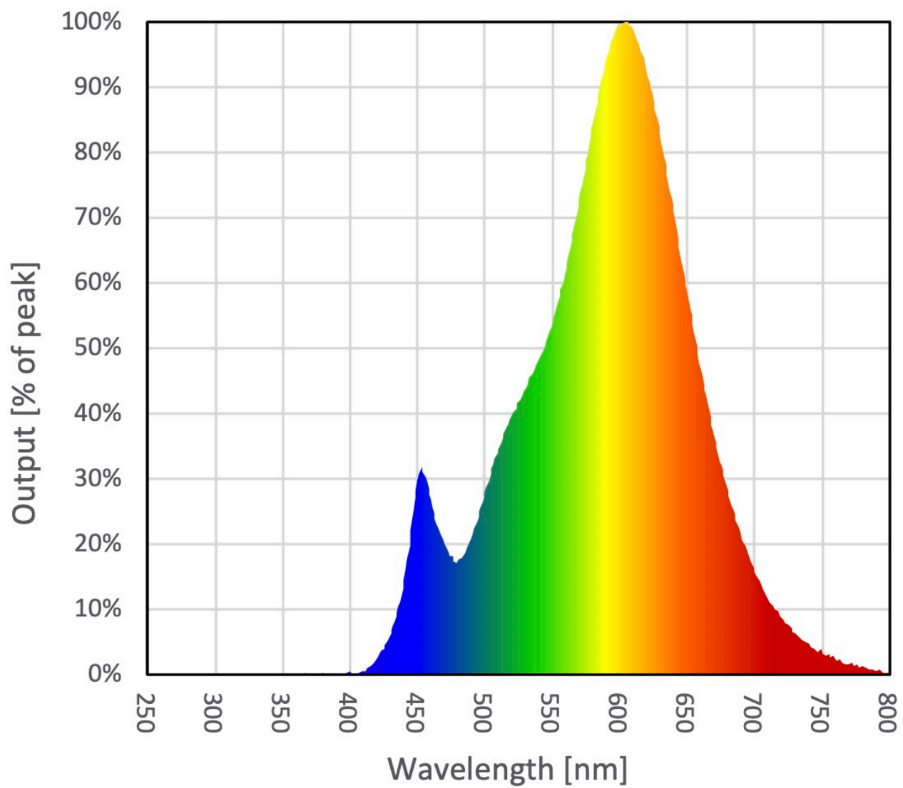
Spectral Power distribution - SP-SWR-G9
