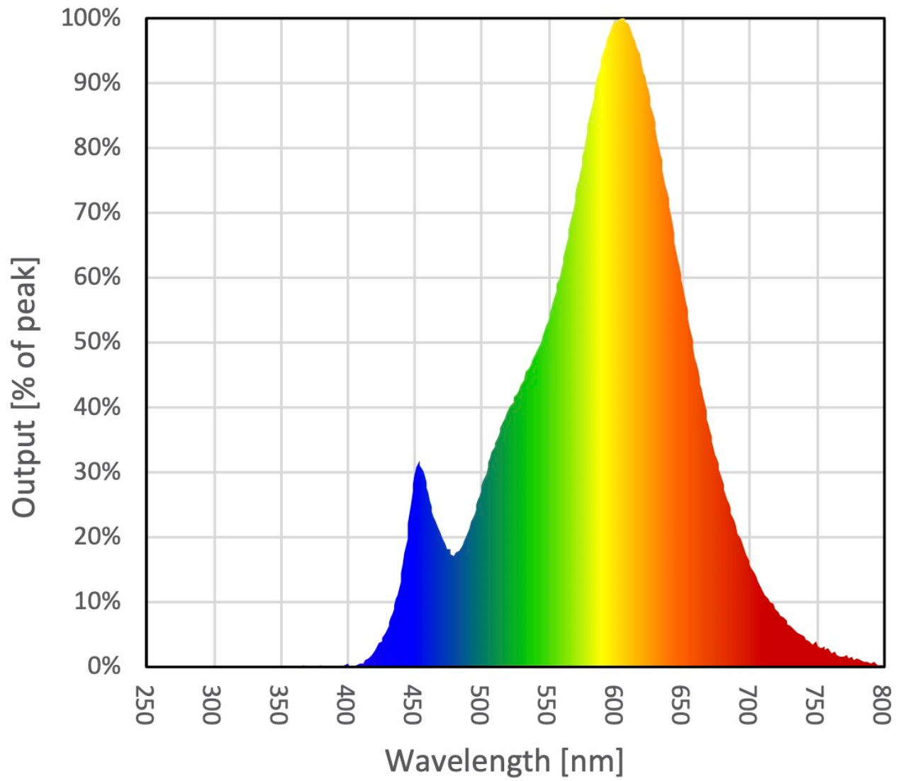
Spectral Power distribution - SP-SWR-G9
