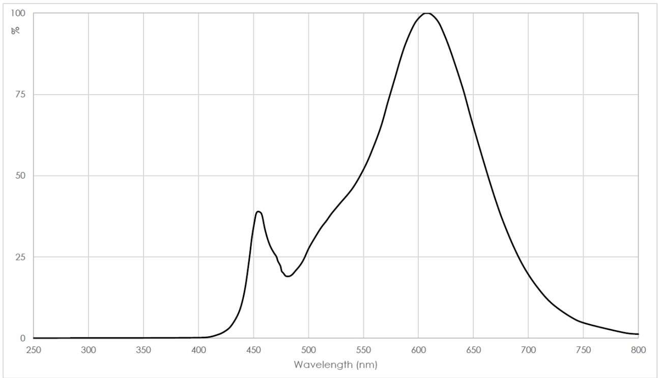
Spectral power distribution - 2700K
