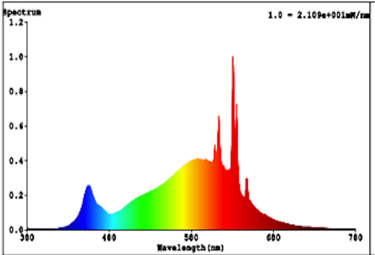
Spectral Distribution
