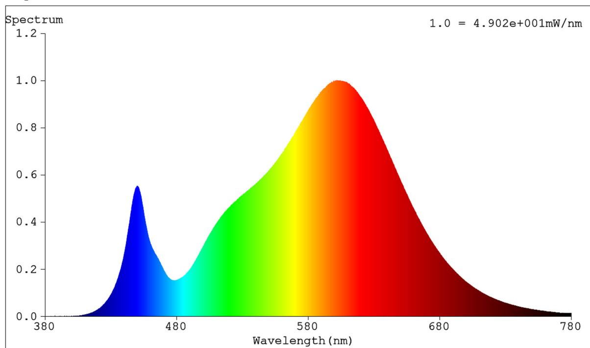
Spectral Distribution
