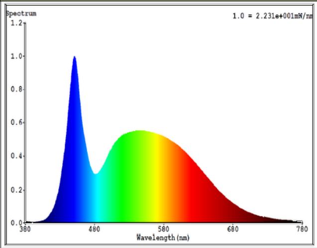
EDE-BAQ501-9W E27 (6500K): 1#
