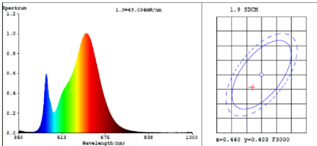
HY-D1200x10x1.2-2C42B-84-1/6 2835-0.5W-vv-8-3000K
