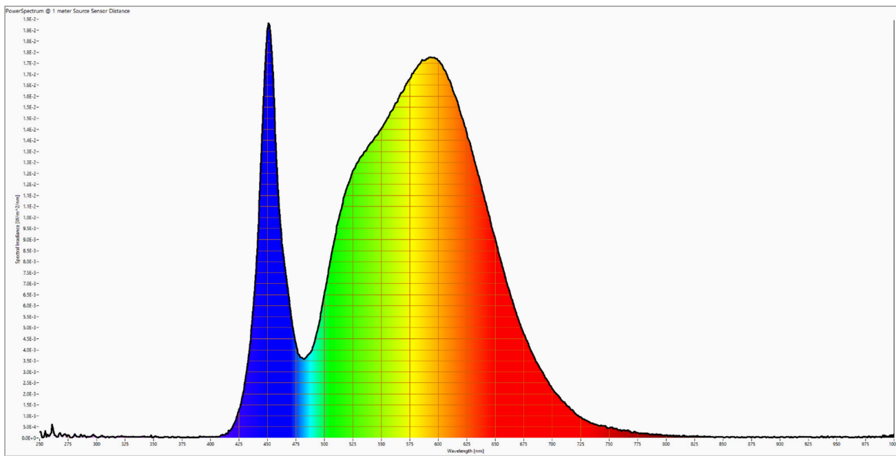
SIGOR-4042301_FULL_powerspectrum_at_1m_distance.png
