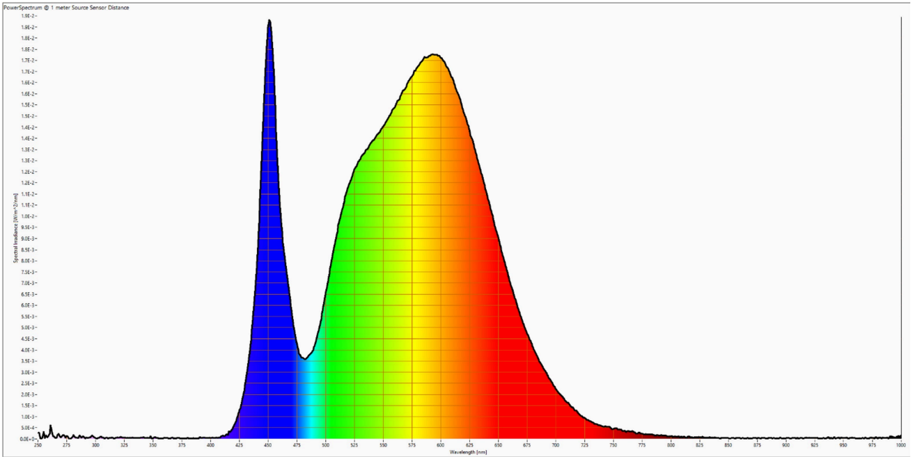
SIGOR-4043101_FULL_powerspectrum_at_1m_distance.png
